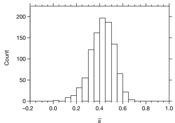
Figure 1 The distribution of 1,000 bootstrap values of \bar{\alpha} for the divergence between Drosophila simulans and D. yakuba for genes in which P_s > 5 . \bar{\alpha} is the average proportion of amino-acid substitutions driven by positive selection.
