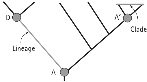
Figure 6.1: The distinction between clades and lineages. A clade is a synchronic, monophyletic set of lineage-representatives, where monophyly is defined synchronically as “all and only descendants of a common ancestor” (represented by A' in this case). A lineage is a diachronic ancestor–descendant connection (between A and D in this case): “species” in the de Queiroz sense.
